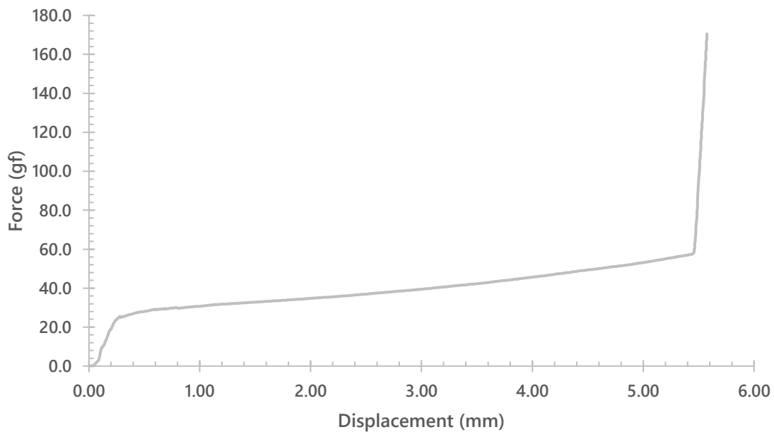
Niz EC Linear UHMWPE 30g (Upstroke)
